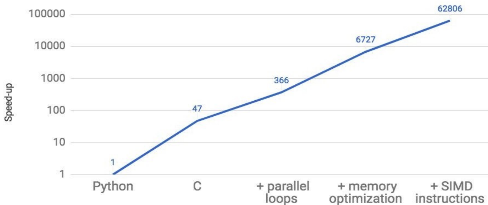
Matrix Multiply Speedup Over Native Python
